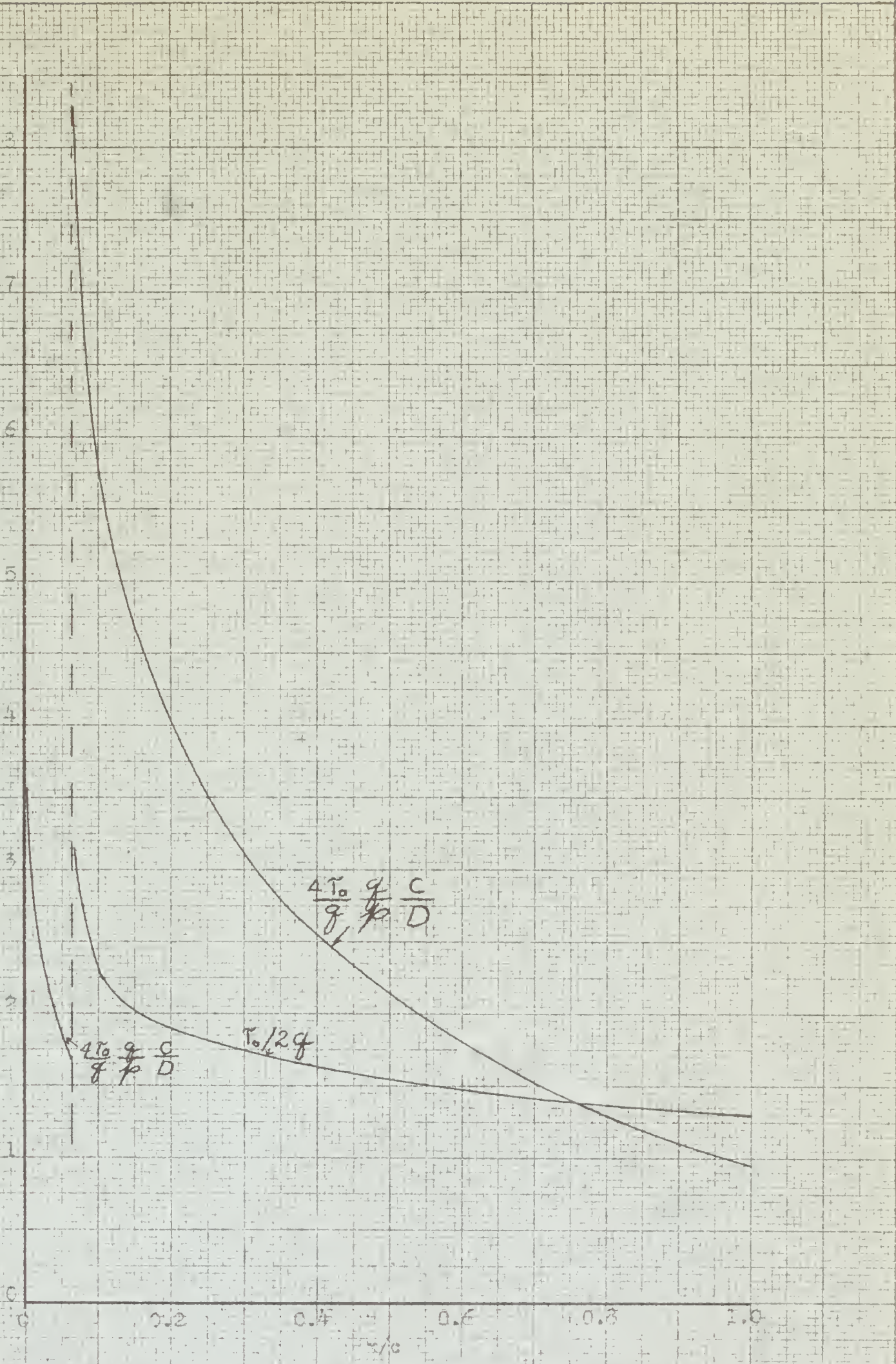
FIG. 21 - FRICTION EFFECTS IN THE CHANNEL.
